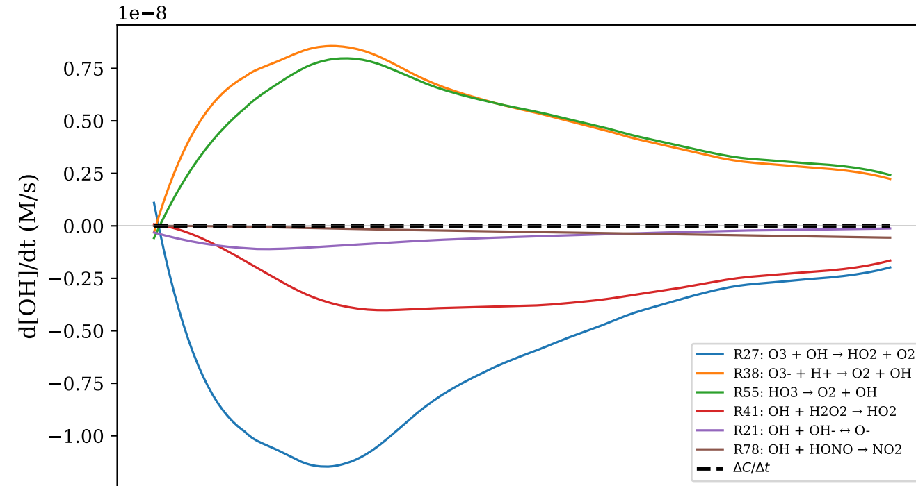
(b) OH [final=0.20 pM]
