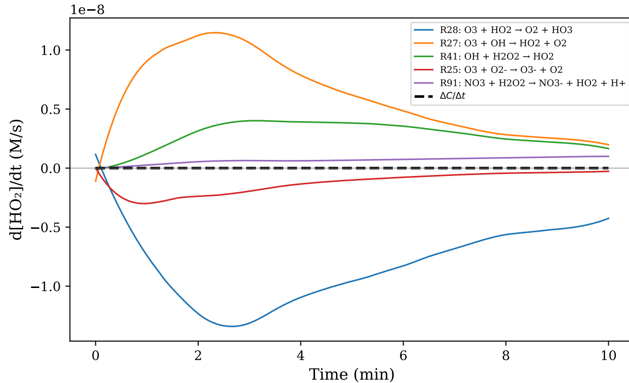
(c) HO 2 [final=292.24 pM]
